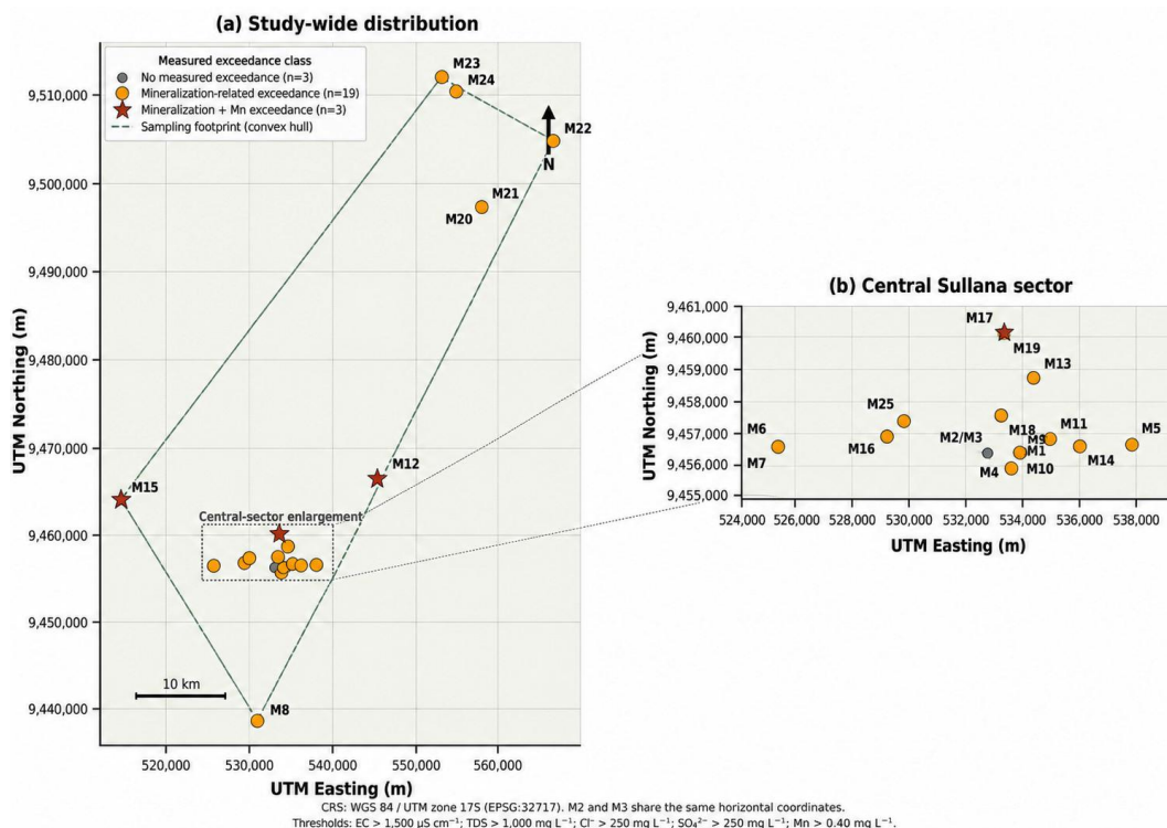
Figure 6. Spatial distribution of measured groundwater-quality exceedances in the Sullana study area. Note. Gray circles show no exceedance, orange circles mineralization, and red stars Mn exceedance. The dashed polygon marks the sampling footprint, not aquifer boundaries. M2–M3 share coordinates; observations do not indicate vulnerability or health risk.
