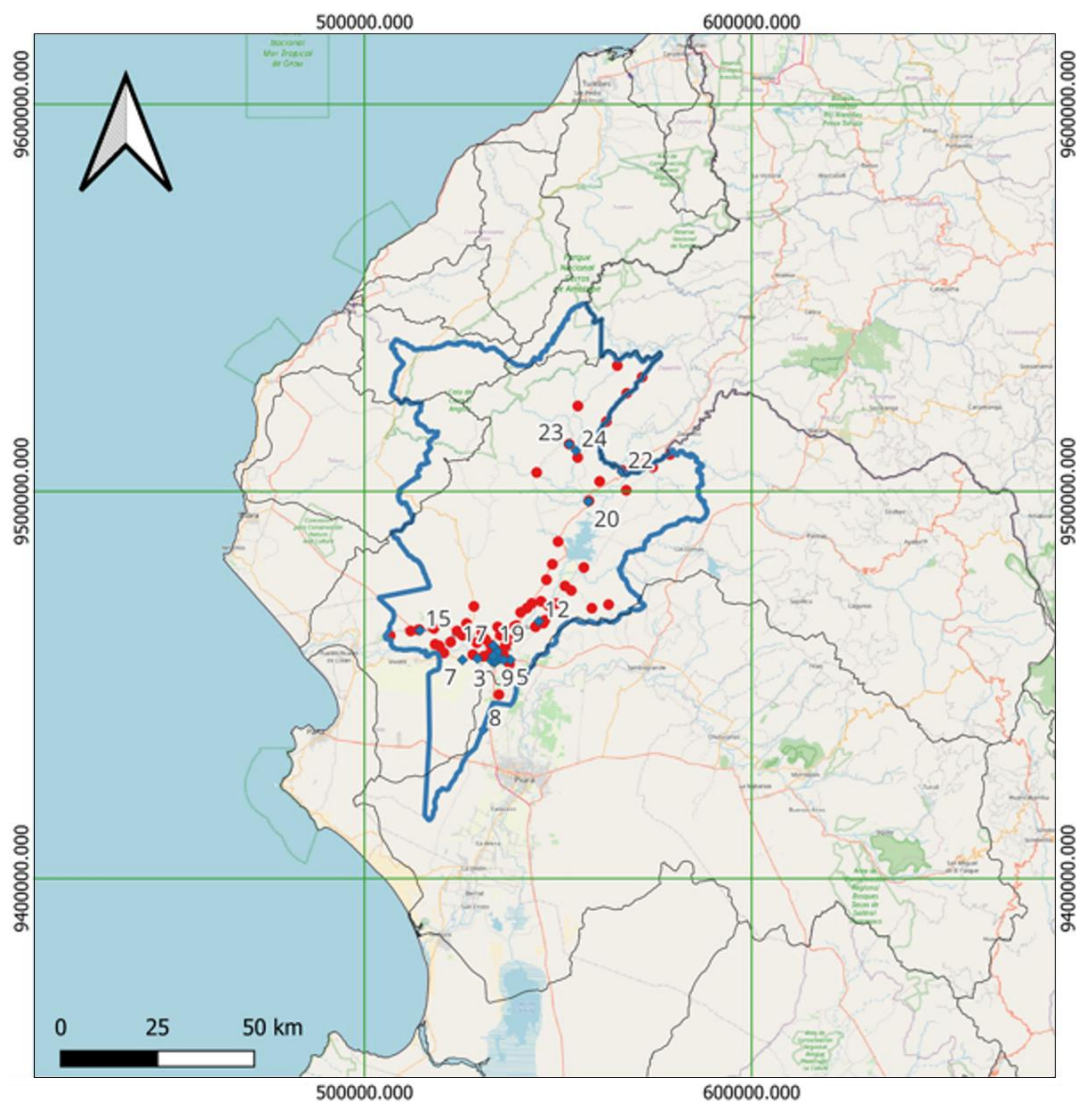
Figure 1. Location of the domain of the Chira groundwater study and spatial distribution of the 25 groundwater sampling sites. Note. Red symbols show wells M1–M25; the blue outline marks the study domain. Coordinates use UTM zone 17M. Symbols indicate sampling locations, not contamination, recharge, vulnerability, or regulatory exceedances.
