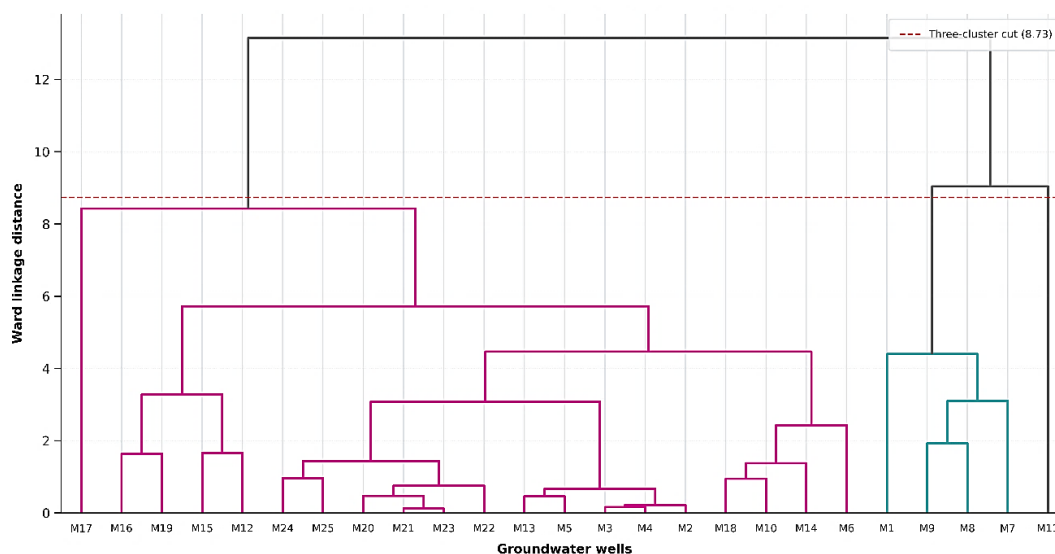
Figure 5b. Dendrogram of the hierarchical cluster analysis of groundwater wells. Note: The dendrogram used nine standardized variables, Euclidean distance, and Ward linkage. Cutting at 8.73 yielded three clusters of 20, four, and one well, representing chemical similarity, not hydrogeological zones.
