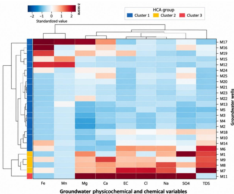
Figure 5c. Heatmap of standardized groundwater physicochemical and chemical variables. Note. Colors show standardized values: warm above-average and cool below-average. Ward clustering orders wells and variables. The side bar identifies three clusters; invariant or censored variables were excluded from analysis.
