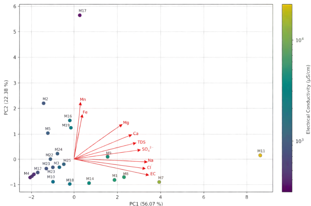
Figure 5a. PCA biplot of groundwater physicochemical and chemical variables. Note: The biplot projects 25 wells and nine variables. PC1 represents mineralization (56.07%); PC2 reflects Fe–Mn variability (22.38%). Together, both explain 78.46%; vector direction and length indicate association and contribution.
