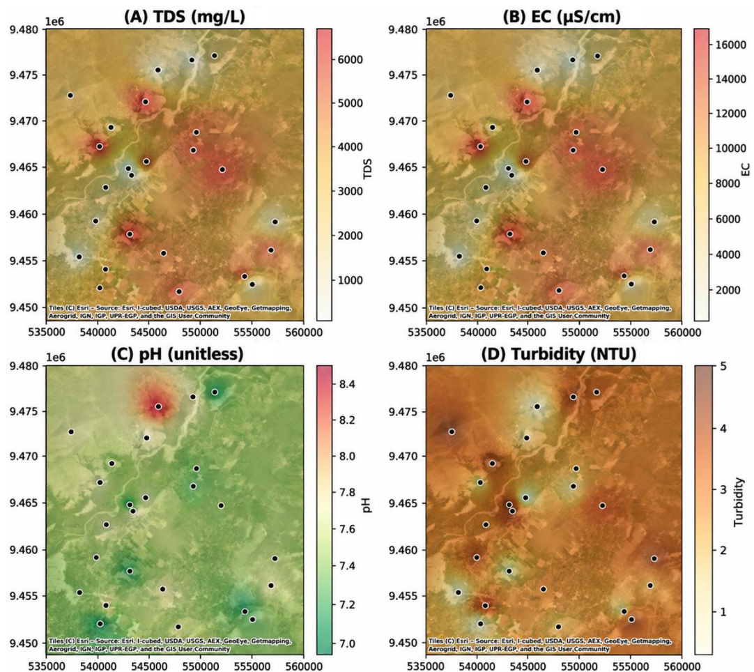
Figure 3. Spatial distribution of selected groundwater physicochemical parameters in the sampled study domain: (A) total dissolved solids, (B) electrical conductivity, (C) pH, and (D) turbidity. Note: IDW used 24 unique locations with p = 2 . M2–M3 parameter means supported interpolation only. Black symbols mark sampled wells; color gradients represent spatial estimates, not measurements or confirmed contamination zones.
