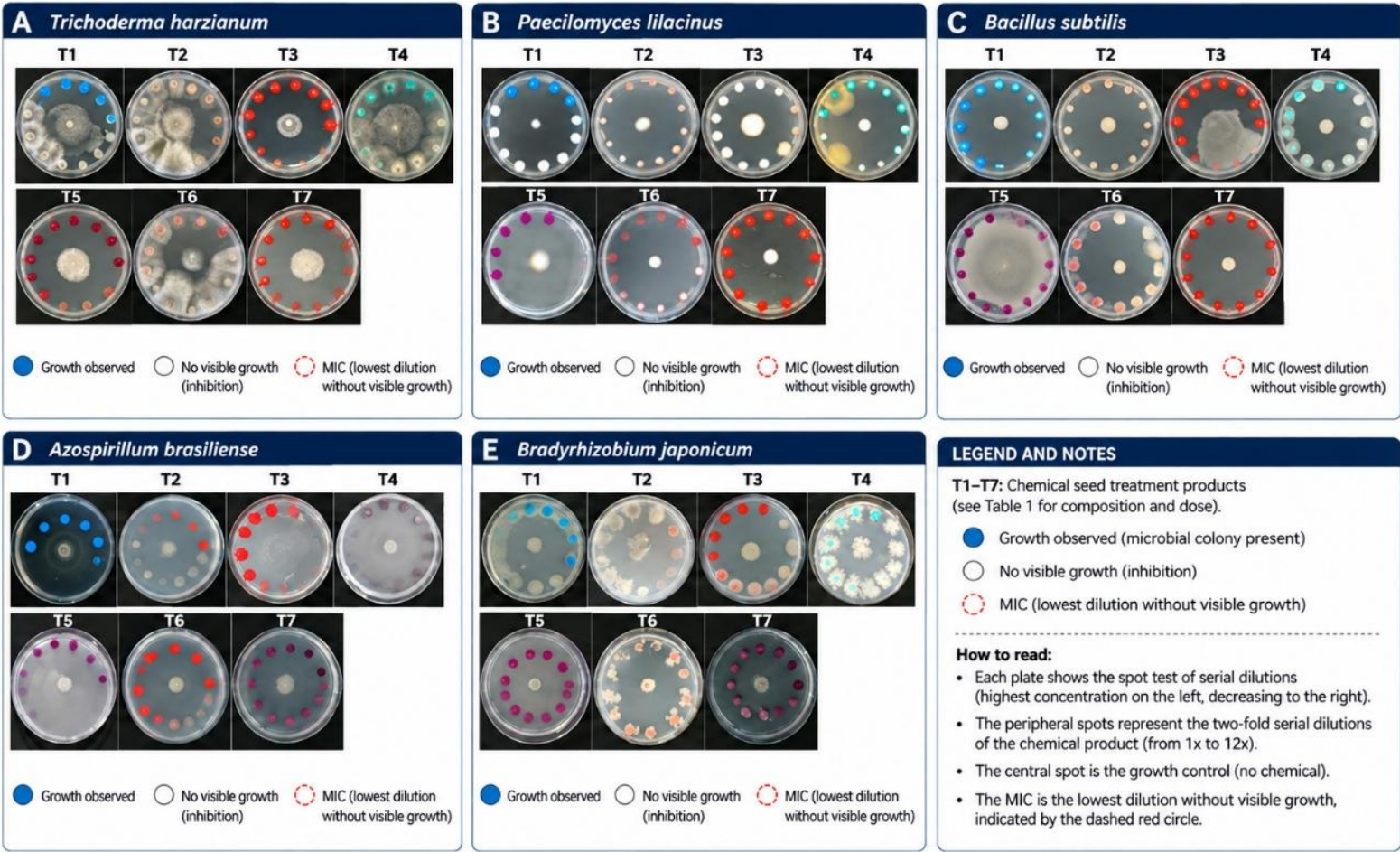
Figure 5. Representative spot-test assay used to confirm the minimum inhibitory concentration (MIC) of chemical seed treatment formulations against beneficial microorganisms. Following serial two-fold microdilution in Brain Heart Infusion (BHI) broth, 10-μL aliquots from each dilution were transferred onto potato dextrose agar (PDA) plates and incubated at 25 ± 2 °C for 48 h. The presence or absence of microbial growth was used to confirm the minimum inhibitory concentration (MIC) for Trichoderma harzianum , Paecilomyces lilacinus , Bacillus subtilis , Azospirillum brasilense , and Bradyrhizobium japonicum . Representative images show the transition between complete growth inhibition and growth recovery across the dilution series of the evaluated chemical seed treatment formulations.
