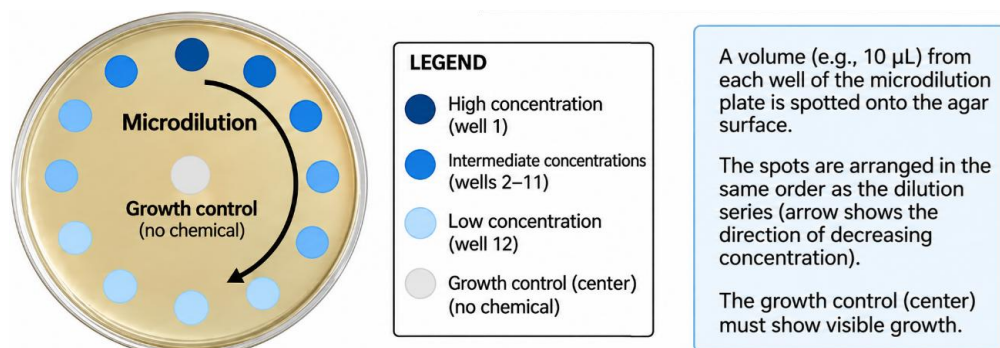
Figure 3. Spot test used to confirm the results of the serial microdilution. The experiment was arranged in a completely randomized design with eight chemical treatments and three replicates for each biological agent.
