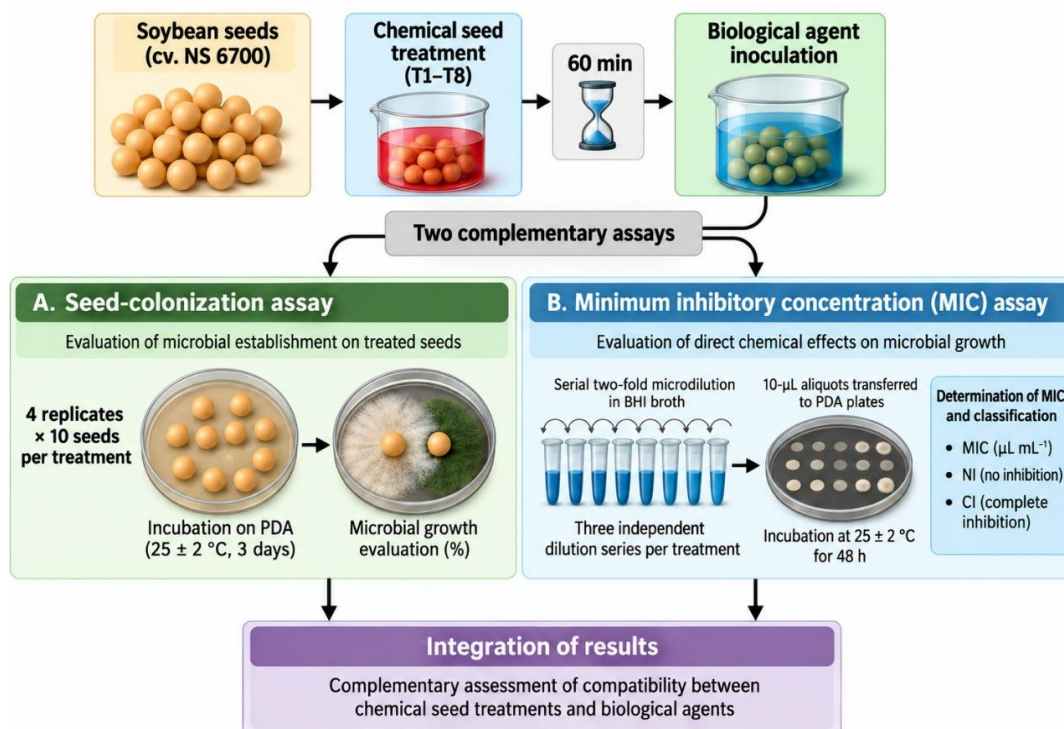
Figure 1. Experimental workflow used to evaluate the compatibility between chemical seed treatments and biological agents. Soybean seeds (cv. NS 6700) were subjected to chemical seed treatment and, after 60 min, inoculated with the biological agents. Two complementary approaches were subsequently performed: (A) a seed-colonization assay to evaluate microbial establishment on chemically treated seeds and (B) a minimum inhibitory concentration (MIC) assay based on serial microdilution followed by spot-test confirmation. The results obtained from both assays were integrated to assess the compatibility between chemical seed treatments and biological agents.
