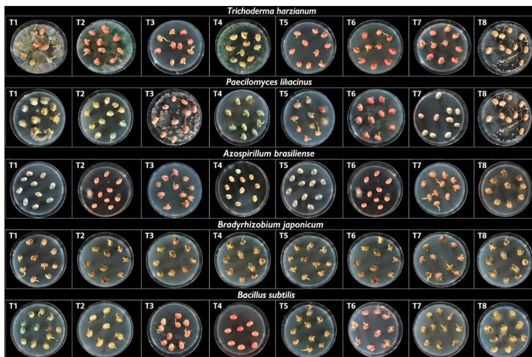
Figure 4. Growth of biological agents on soybean seeds subjected to different chemical seed treatments. Soybean seeds were treated with chemical products (T1–T7) or left untreated (T8) and subsequently inoculated with the biological agents Trichoderma harzianum , Paecilomyces lilacinus , Bacillus subtilis , Azospirillum brasilense , and Bradyrhizobium japonicum . Seeds were incubated on potato dextrose agar (PDA) medium for three days at 25 \pm 2^\circ\text{C} , and microbial growth was assessed under a stereomicroscope (80× magnification). Images represent the visual response of each biological agent to the chemical seed treatments, demonstrating differences in microbial colonization and growth among treatments.
