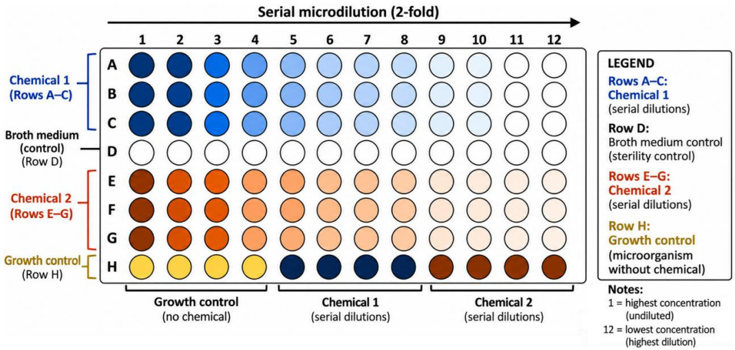
Figure 2. Serial microdilution setup used to determine the minimum inhibitory concentration (MIC).
